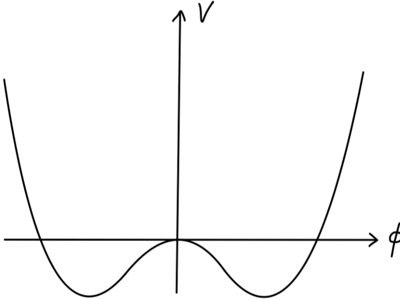
Figure 3.2: Standard Model
